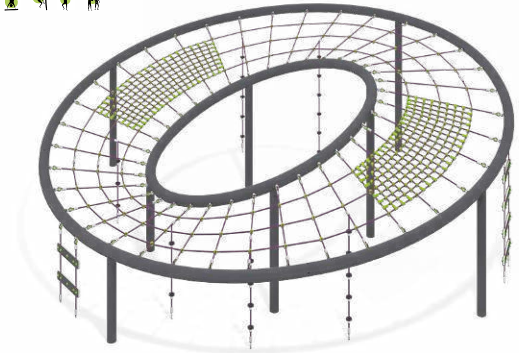
21.019 Rope Climbing Playground Baikal width length height fall height 6 170 mm 6 250 mm 2 100 mm 2 100 mm Age range: 7-12 years
